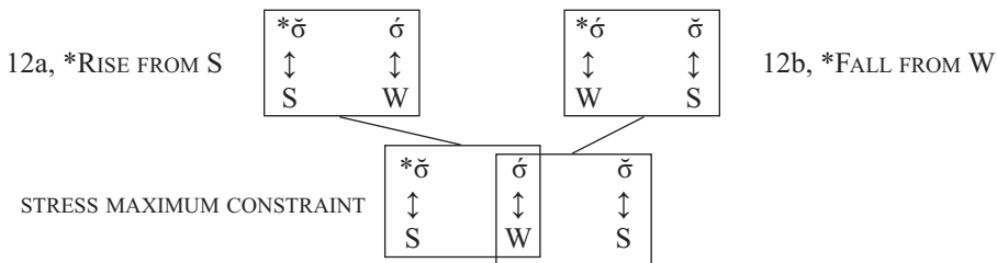
FIGURE 4. The stress maximum constraint as local conjunction.
